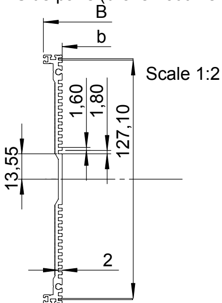
Side panel(broken out view) MAXI 3-all
