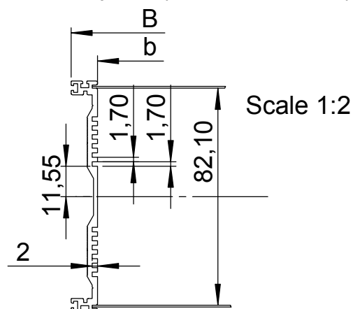
Side panel(broken out view) MAXI 2-all
